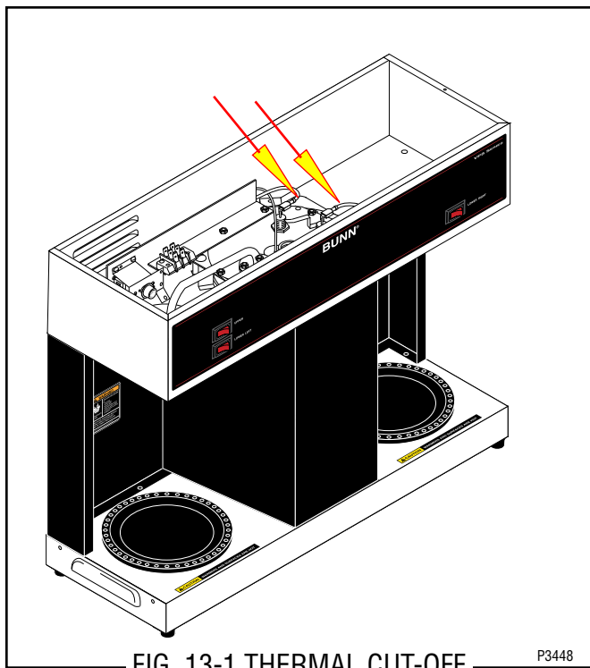
FIG. 13-1 THERMAL CUT-OFF
