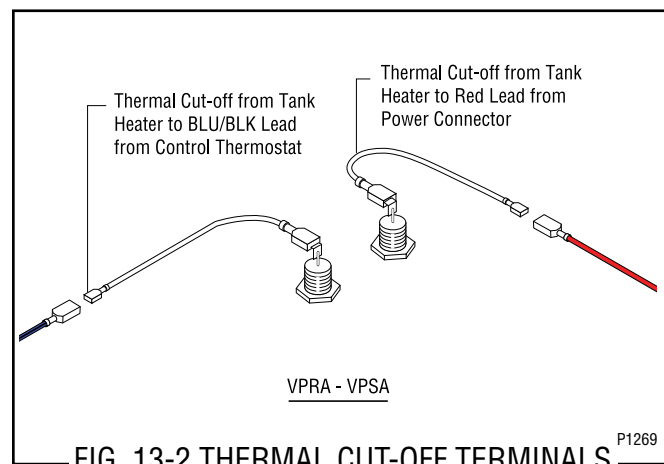
FIG. 13-2 THERMAL CUT-OFF TERMINALS
