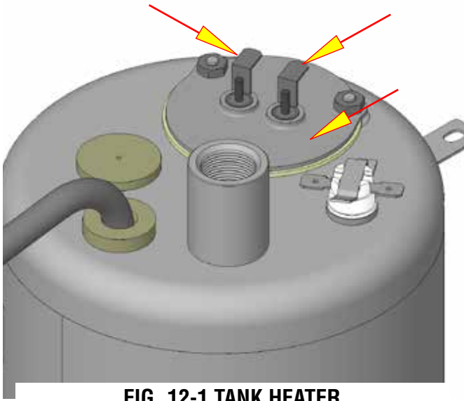
FIG. 12-1 TANK HEATER
