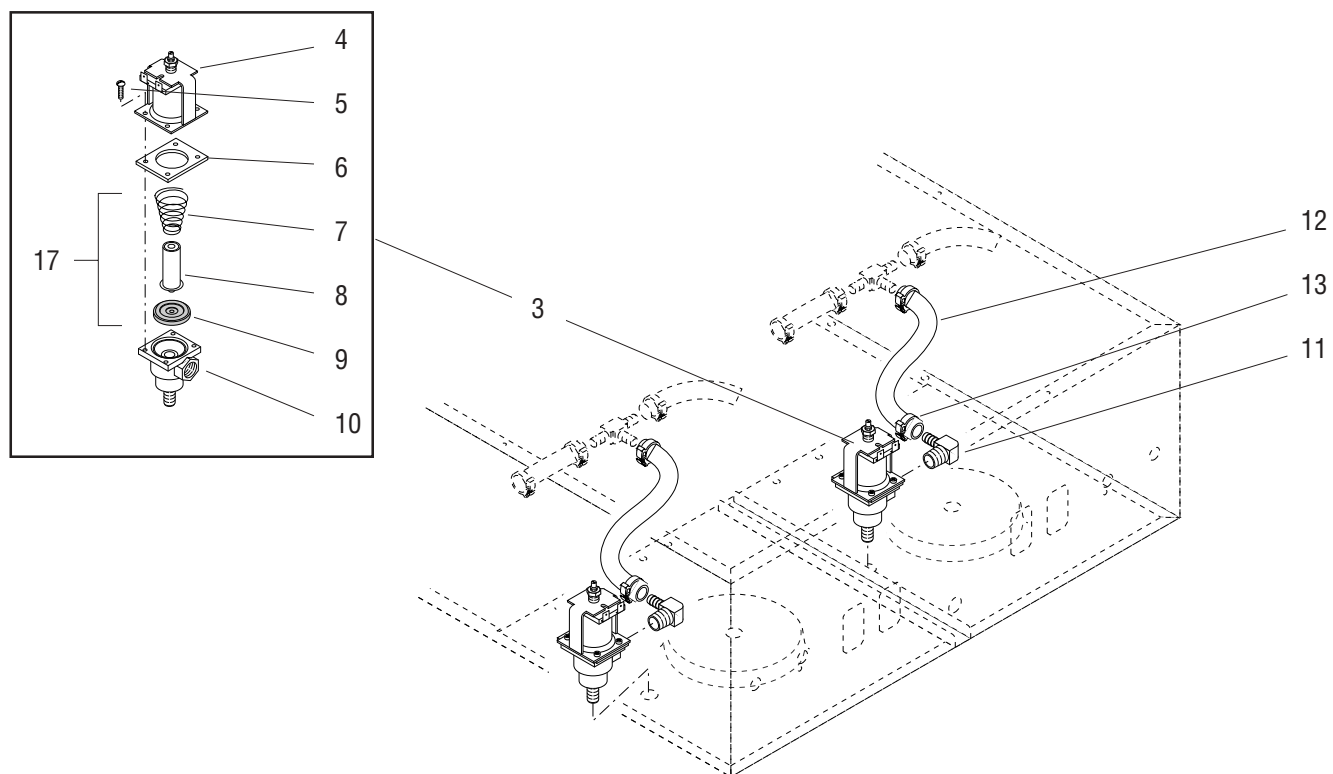
ELECTRO / MECHANICAL BY-PASS
